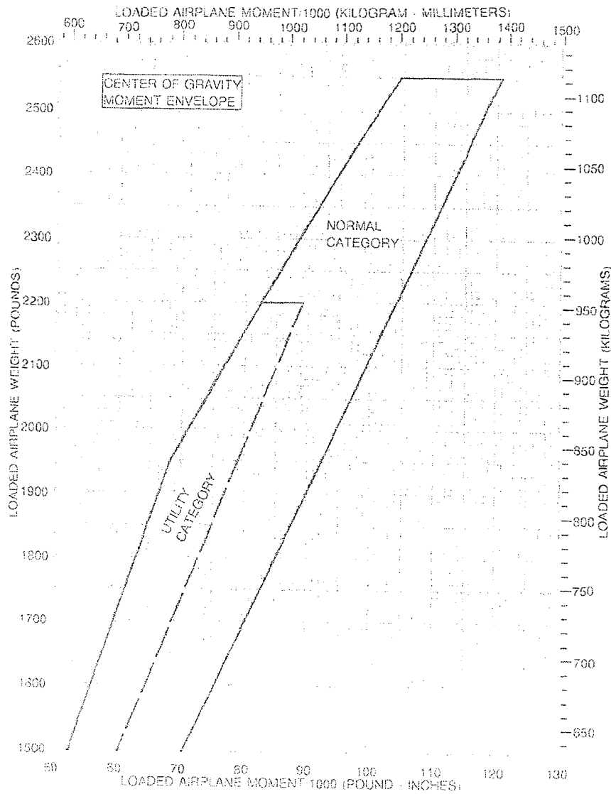
Figure 19 Center of Gravity Moment Envelope
