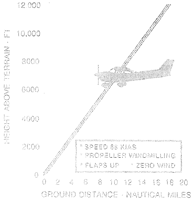
Figure 4 Maximum Glide
