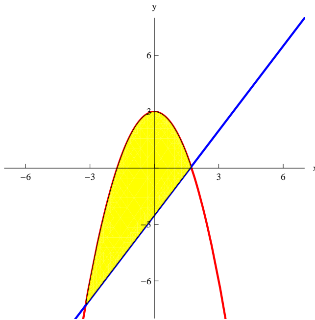
FIGURE 1. Solution is the yellow shaded region between the two graphs
